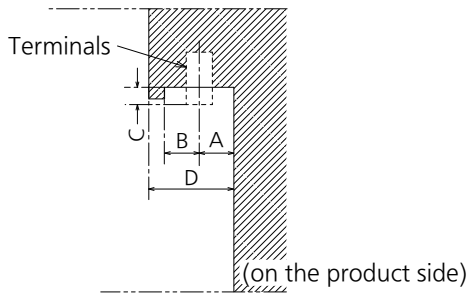
Sectional view of terminal a (AUDIO IN / AUDIO OUT / VIDEO AV IN / SERIAL IN / PC IN / DVI-D IN)
